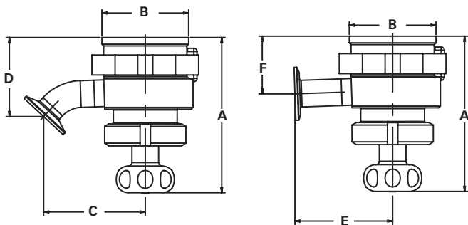
Flush Mounted Radial Diaphragm Valve
