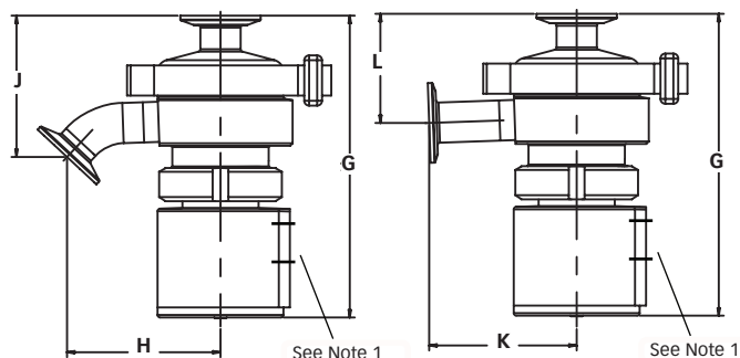
Actuated Clamp Mounted Radial Diaphragm Valves
